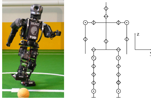
Autonomous humanoid robot Bruno kicking a ball (left, with designed head) and kinematical structure of the robot (right).
